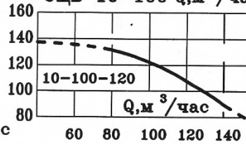
ЭЦВ 10-100 Q, \text{ м}^3/\text{час}
